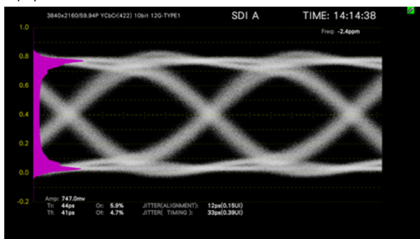
Eye pattern
